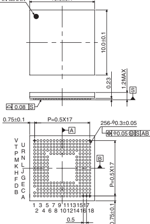
VBGA256T100
