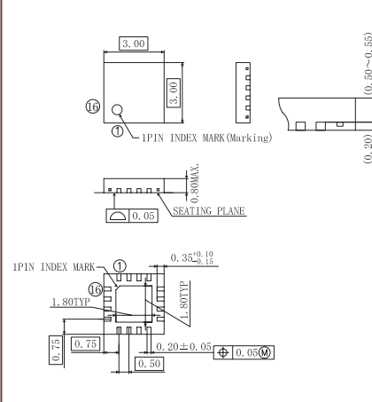
WQFN16-0303-0.50
