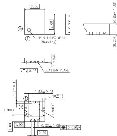
WQFN12
