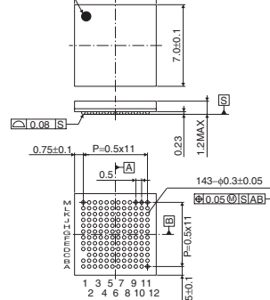
VBGA143T070
