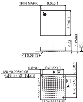
VBGA120T060
