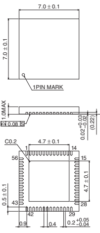
UQFN056V7070
