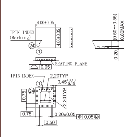
WQFN24
