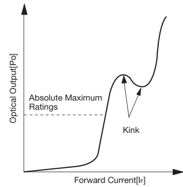
■ Fig.1 Optical Output vs. Forward Current
