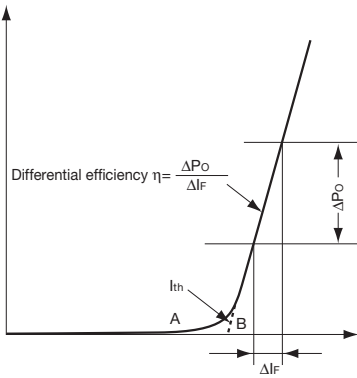
Fig.2 Optical Output vs. Forward Current
