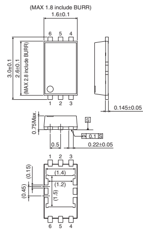
Embossed carrier tape:3,000pcs
