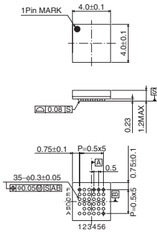
VBGA035T040
