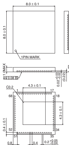
UQFN068V8080
