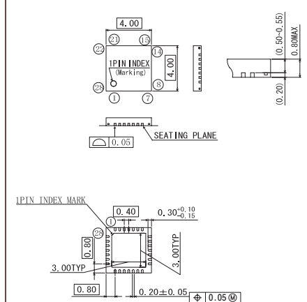
P-WQFN28-0404-0.40-63
