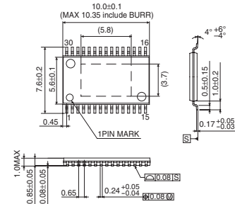
HTSSOP-B30
