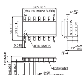
SOP-J14
