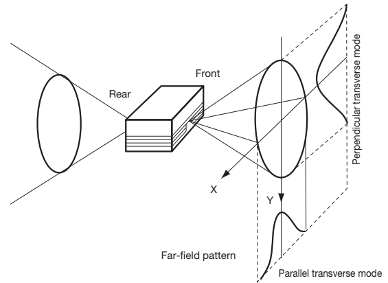
Fig.3 Radiation Characteristics
