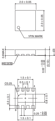
VSON008X2020
