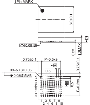
VBGA099T060
