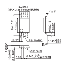
TSSOP-B8
