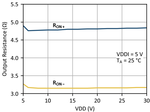
Figure 28. Output Resistance vs. Gate Driver Supply Voltage
