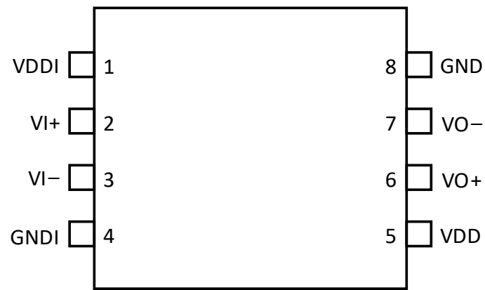
Figure 3. Si82A40x Pinout
