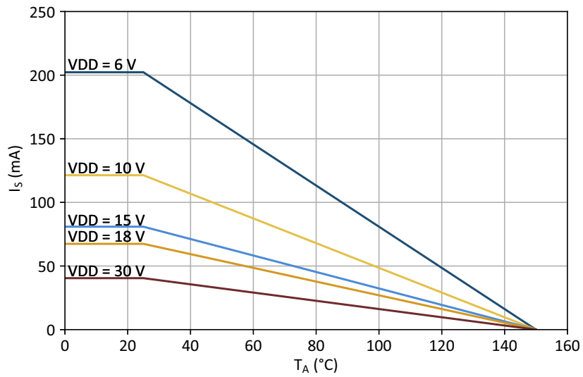
Figure 33. SSO-8 Safety Current vs. Ambient Temperature Derating Curve
