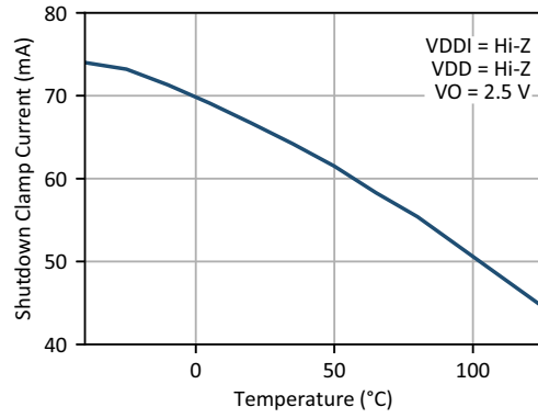
Figure 31. Shutdown Clamp Current vs. Ambient Temperature
