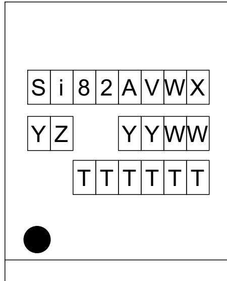
Figure 39. 8-Pin Stretched Small Outline (SSO) Top Marking
