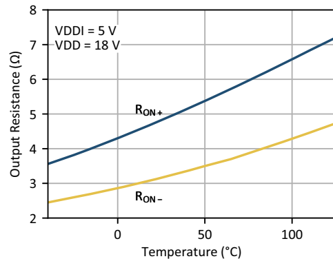
Figure 29. Output Resistance vs. Ambient Temperature
