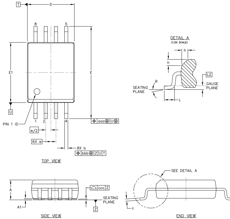
Figure 35. SSO-8 Package Drawing
