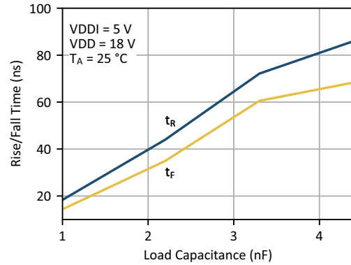
Figure 25. Output Rise/Fall Time vs. Output Load
