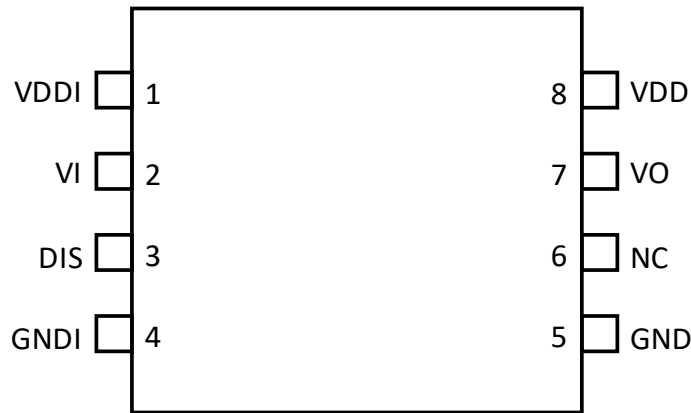
Figure 1. Si82A28x Pinout
