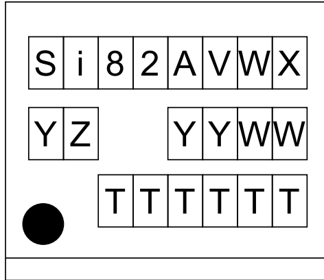
Figure 38. 8-Pin Narrow-Body SOIC Top Marking
