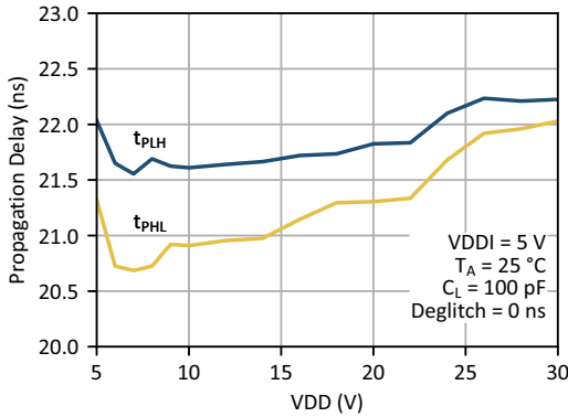
Figure 18. Propagation Delay vs. Gate Driver Supply Voltage
