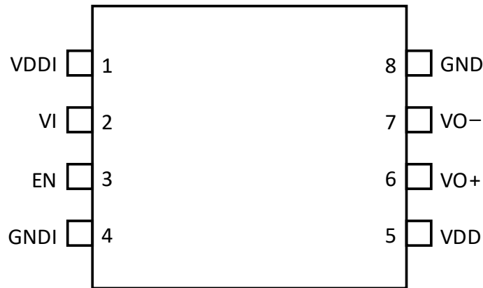
Figure 2. Si82A30x Pinout
