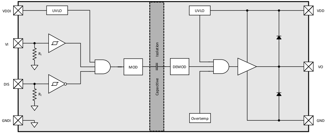
Figure 7. Si82A28x Device with Single Output and Disable Input
