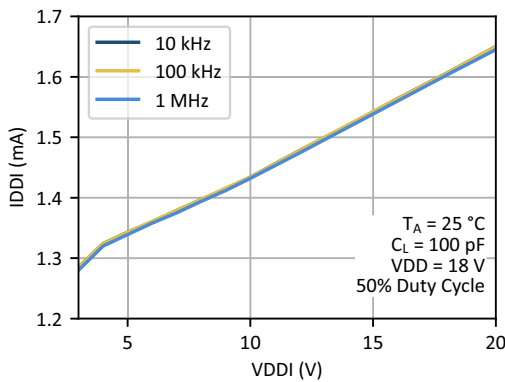
Figure 20. Logic Input Active Supply Current vs. Logic Input Supply Voltage
