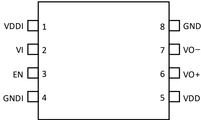
Figure 4. Si82A30x Pinout
