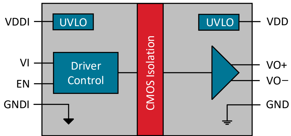
Si82A30x
