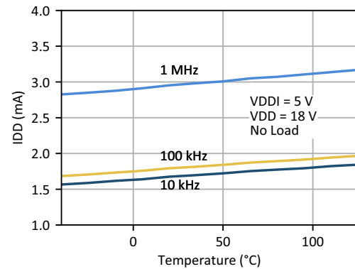
Figure 23. Gate Driver Active Supply Current vs. Ambient Temperature
