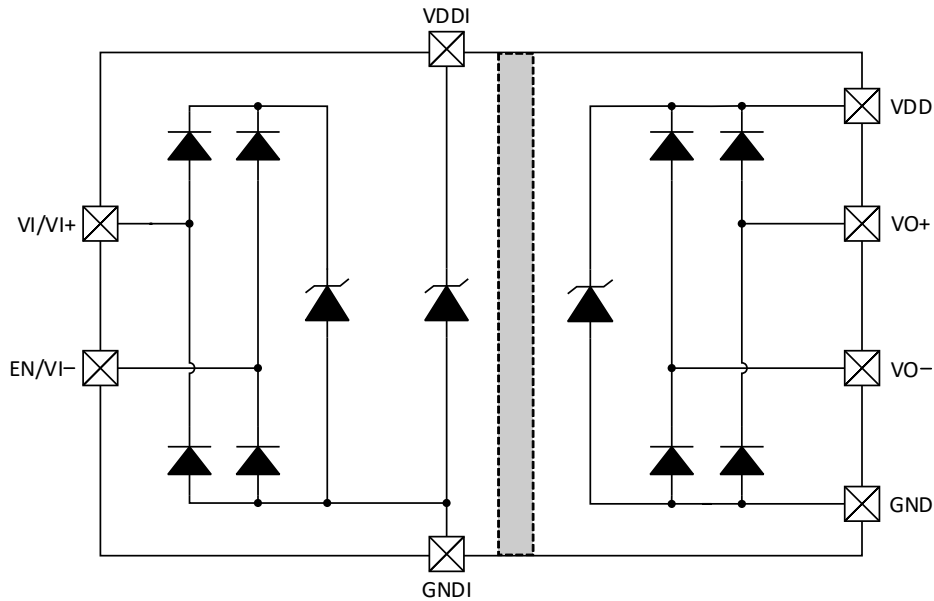
Figure 12. Si82A30x/40x/43x Device ESD Structure
