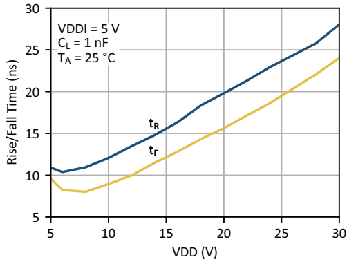
Figure 24. Output Rise/Fall Time vs. Gate Driver Supply Voltage
