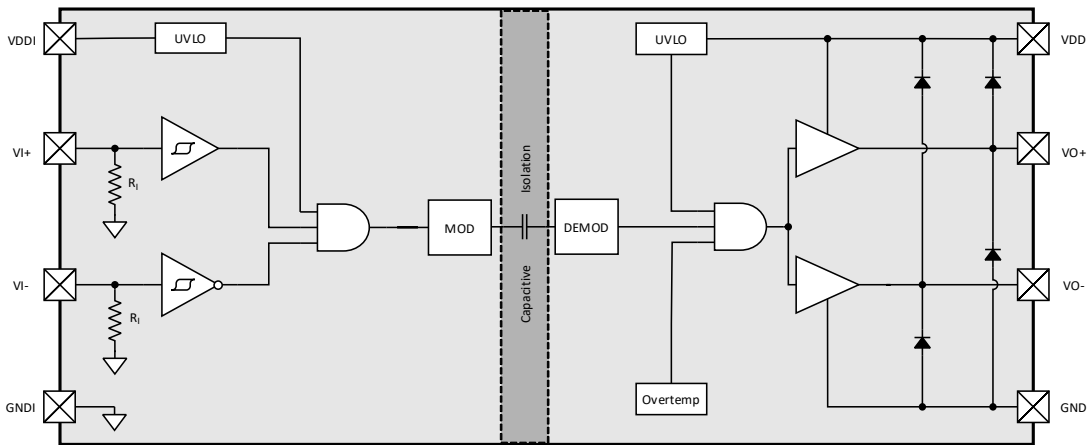
Figure 9. Si82A40x/43x Device with Split Output and Complementary Input
