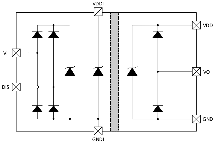
Figure 11. Si82A28x Device ESD Structure
