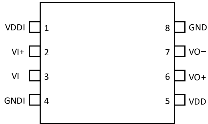
Figure 5. Si82A40x Pinout
