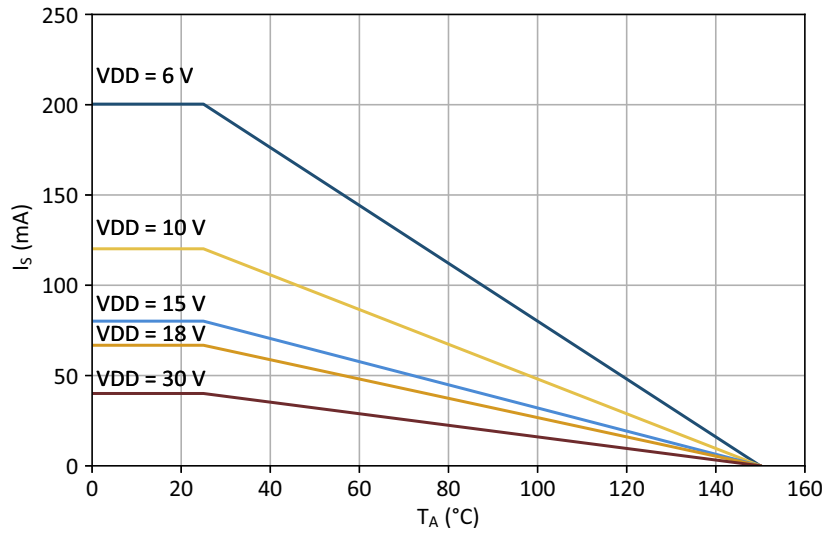
Figure 32. NB SOIC-8 Safety Current vs. Ambient Temperature Derating Curve
