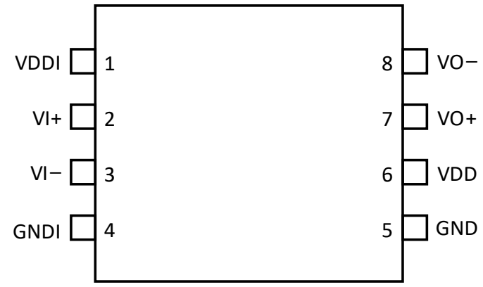
Figure 6. Si82A43x Pinout
