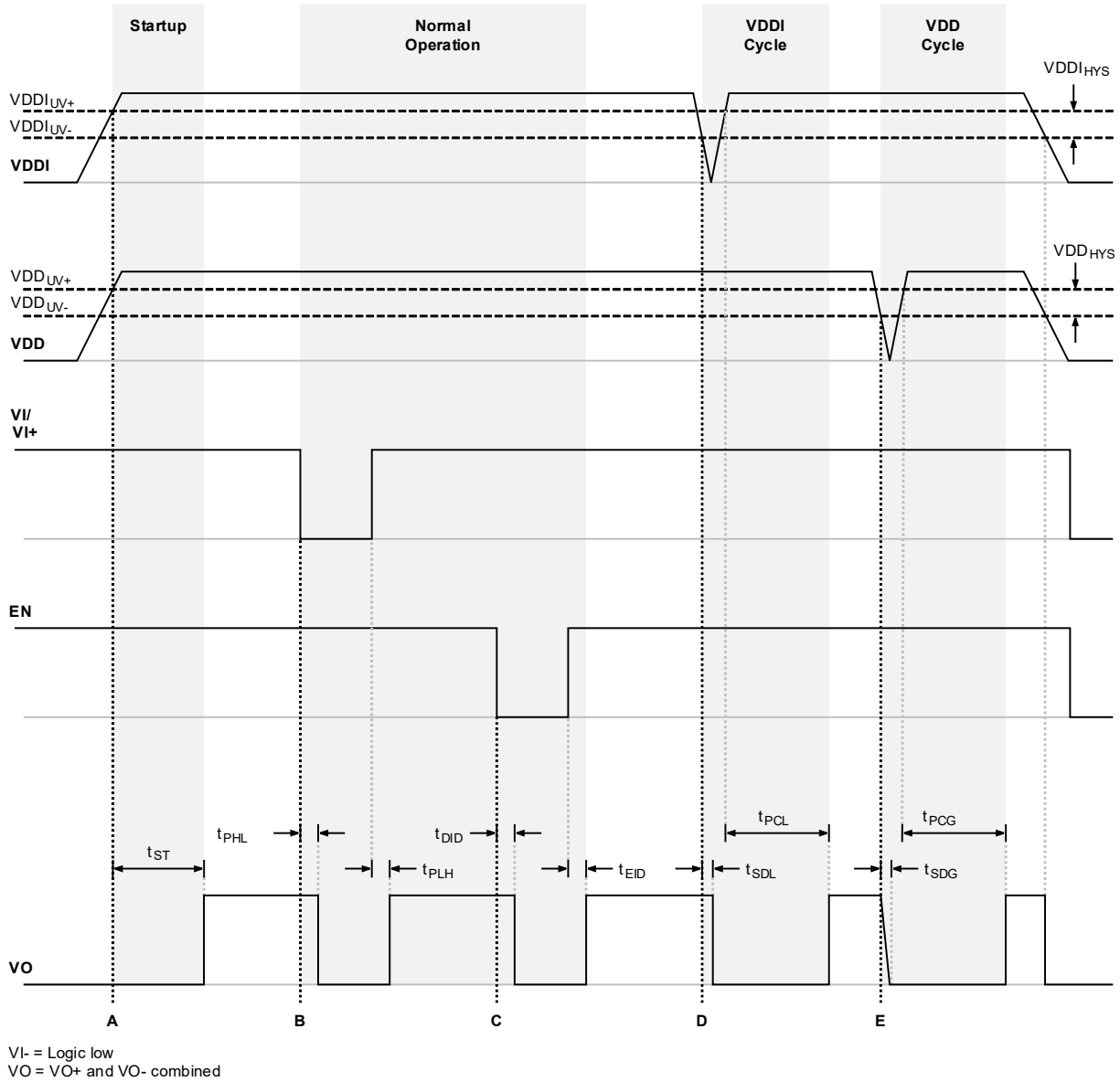
Figure 10. Gate Driver Timing Behavior
