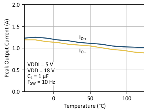
Figure 27. Peak Output Current vs. Ambient Temperature
