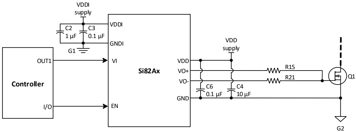
Figure 14. Si82Ax Split Output Application
