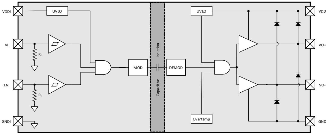
Figure 8. Si82A30x Device with Split Output and Enable Input
