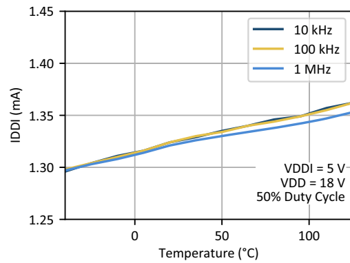
Figure 21. Logic Input Active Supply Current vs. Ambient Temperature
