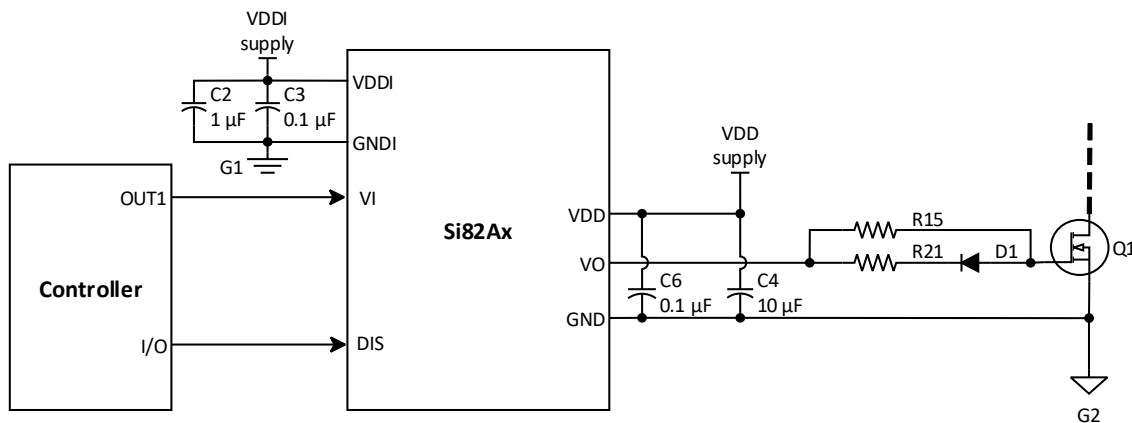
Figure 13. Si82Ax Single Supply Application
