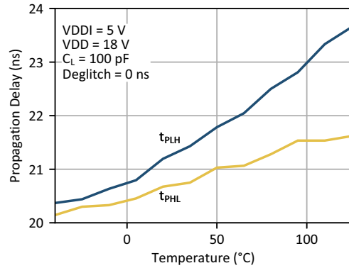
Figure 19. Propagation Delay vs. Ambient Temperature
