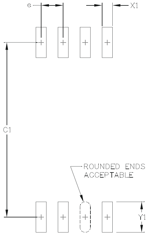
Figure 37. SSO-8 PCB Land Pattern
