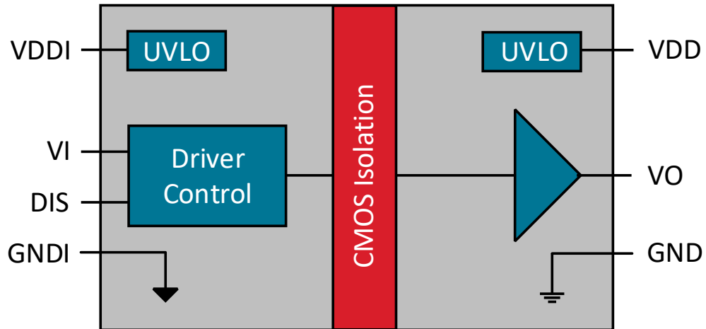
Si82A28x
