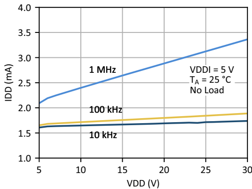
Figure 22. Gate Driver Active Supply Current vs. Gate Driver Supply Voltage
