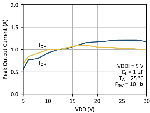
Figure 26. Peak Output Current vs. Gate Driver Supply Voltage
